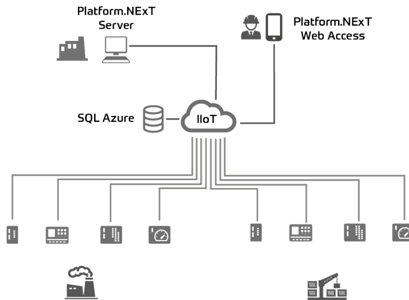
This diagram shows an example of data gathering from various field devices, connected in a single-protocol architecture for IIoT. The data gathering database in the example is Cloud-based (Ms SQL Azure)
